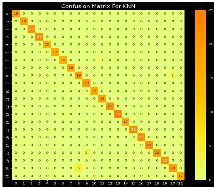
Figure 11. Confusion matrix for KNN.
